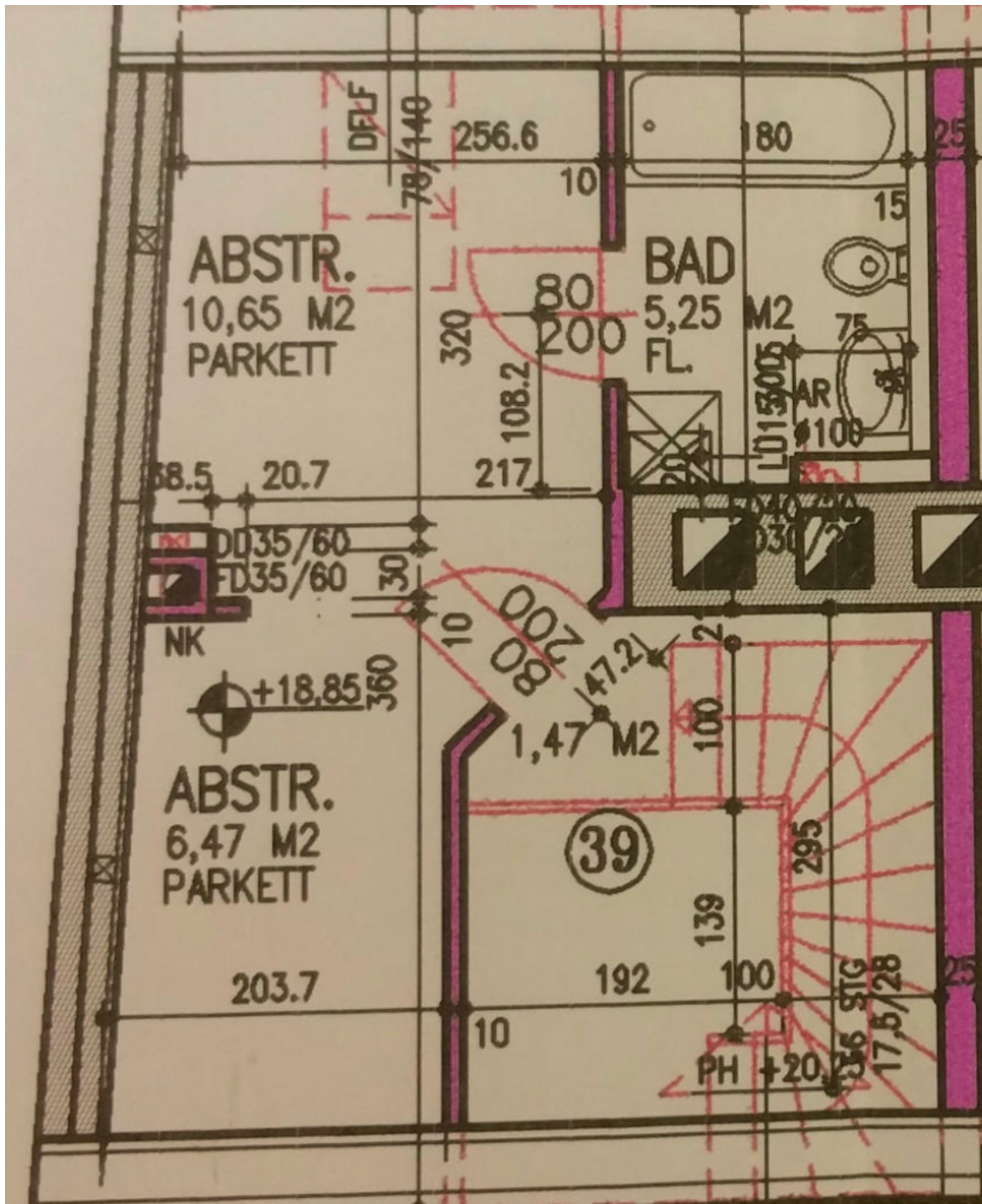
Plan Ebene 2
