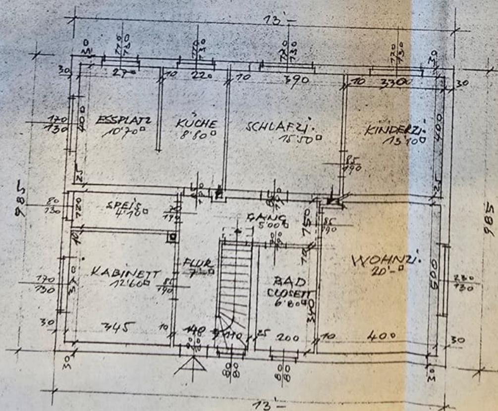
ERDGESCHOSS.
