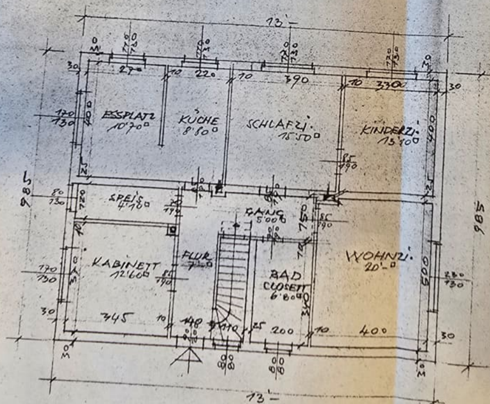
ERDGESCHOSS.
